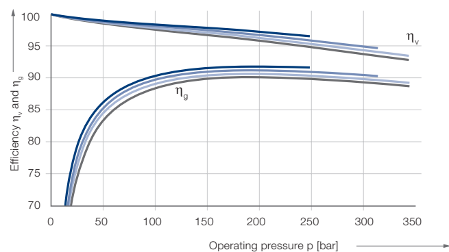
IPVP 5 – Efficiency \eta_v and \eta_g
