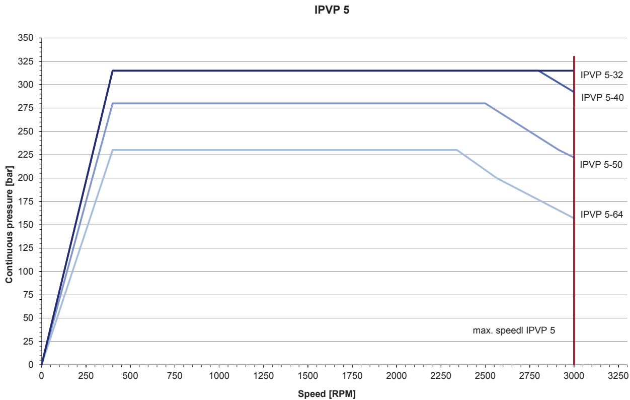
Diagram IPVP 5 - Continuous pressure depending on the speed
