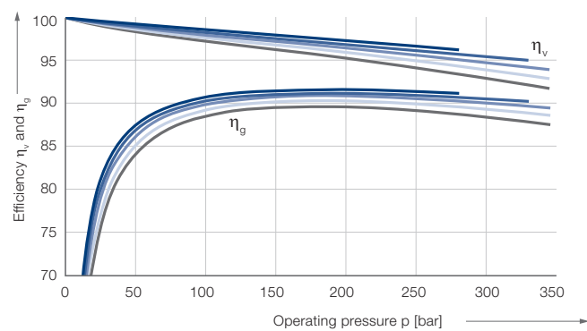
IPVP 4 – Efficiency \eta_v and \eta_g
