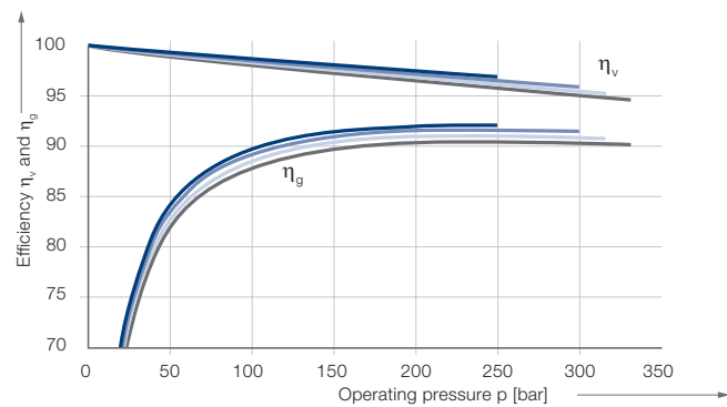
IPVP 7 – Efficiency \eta_v and \eta_g
