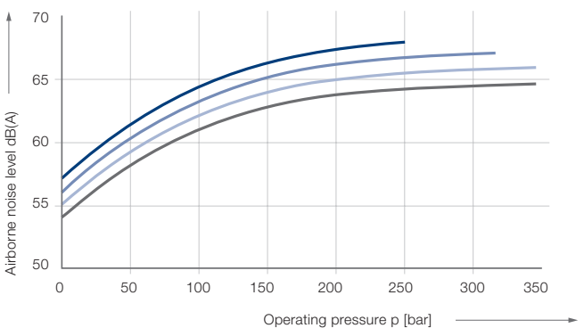
IPVP 5 – Airborne noise level (measuring location 1 m axial)
