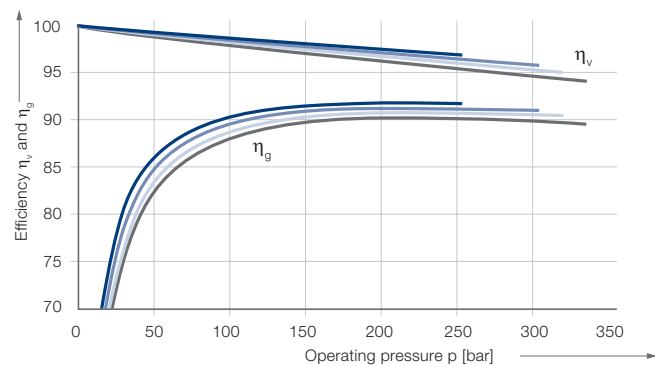
IPVP 6 – Efficiency \eta_v and \eta_g
