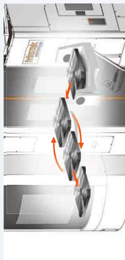
VARIAXIS J-600/5X 2 pallet changer
