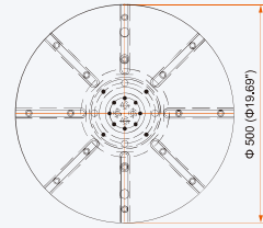
VARIAXIS J-500 VARIAXIS J-500/5X Table dimensions
