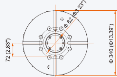
VARIAXIS J-500 VARIAXIS J-500/5X Table dimensions
