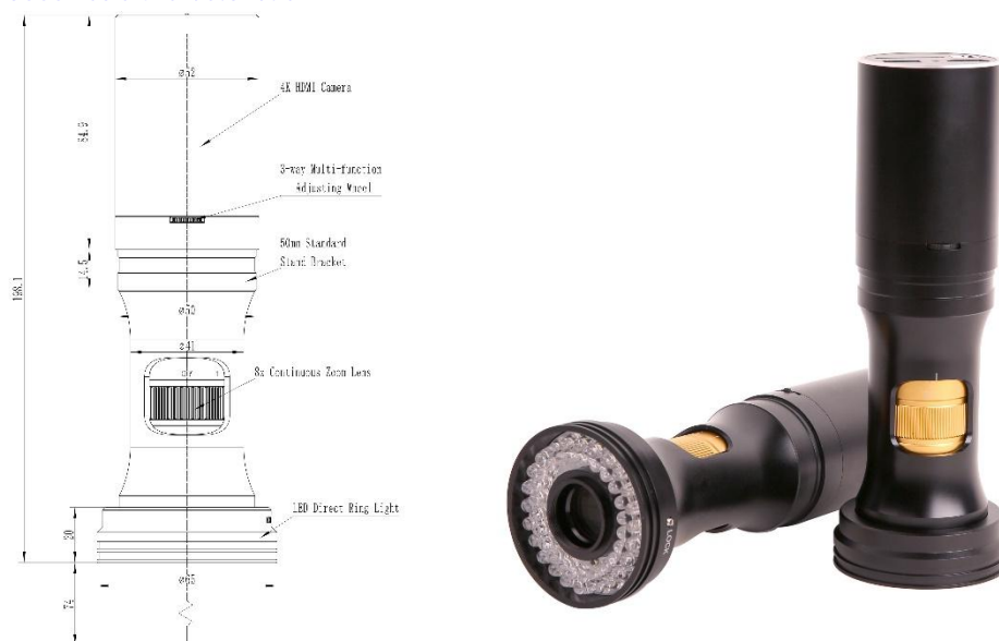
Figure 1. The main body of IZM3000
