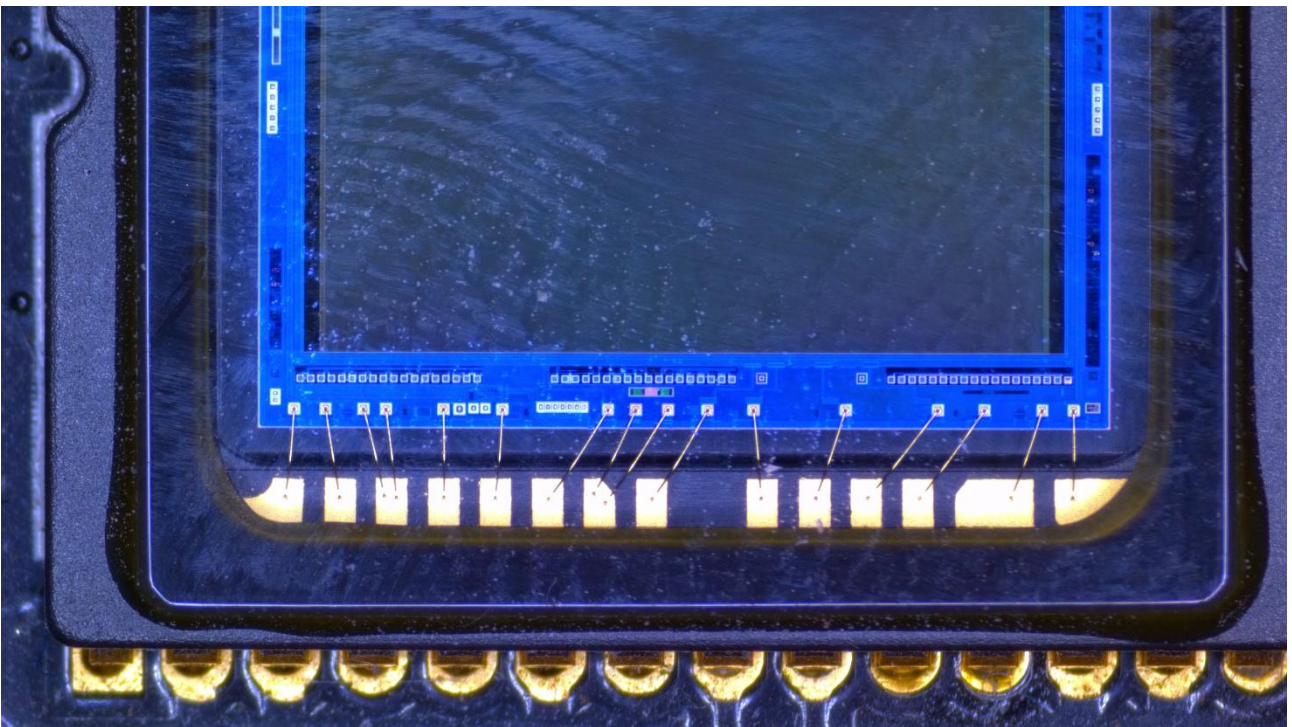
Figure 19. CCD Circuit board captured with IZM3000
