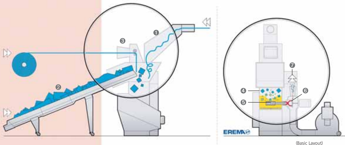
(Basic Layout)
