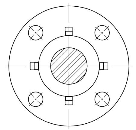
GLAND RING END VIEW
