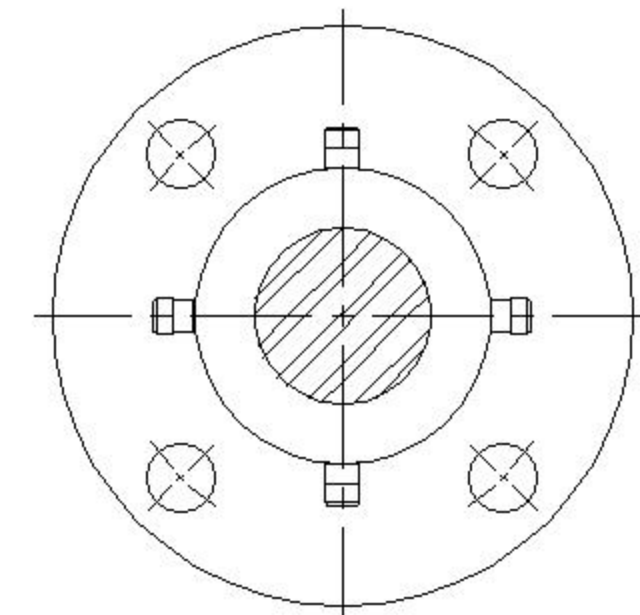
GLAND RING END VIEW
