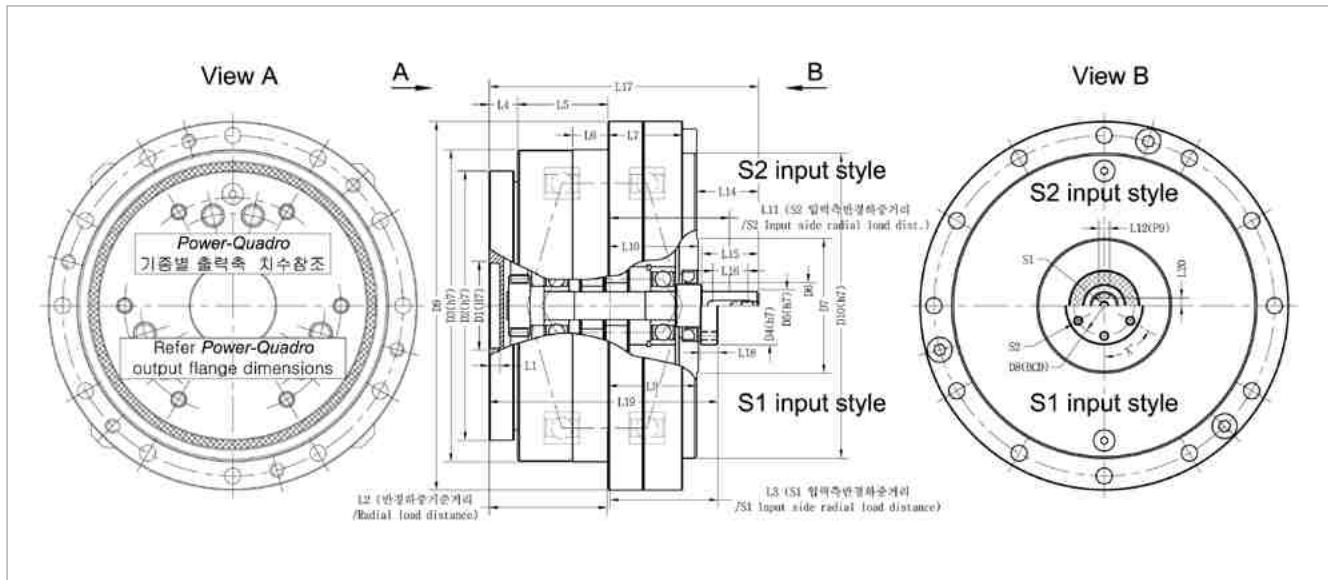
▶ PQ-S1, S2 입력형상치수표 III [PQ-S1, S2 input style dimensions III] (mm)
