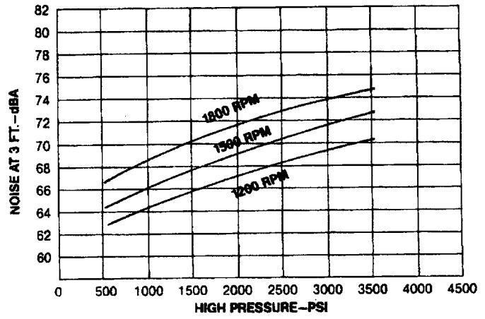
PVWH-10—FULL STROKE
