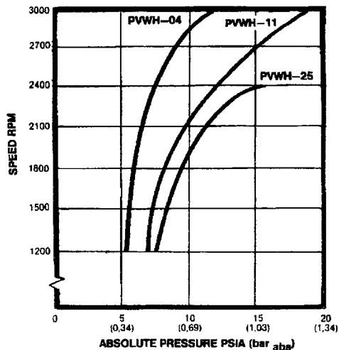
INLET SUCTION/SUPERCHARGE
