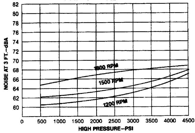
PVWH-06—FULL STROKE
