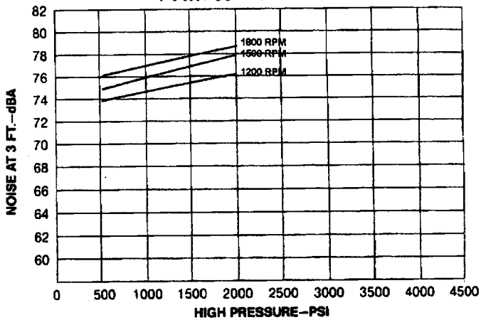
PVWH-60—FULL STROKE
