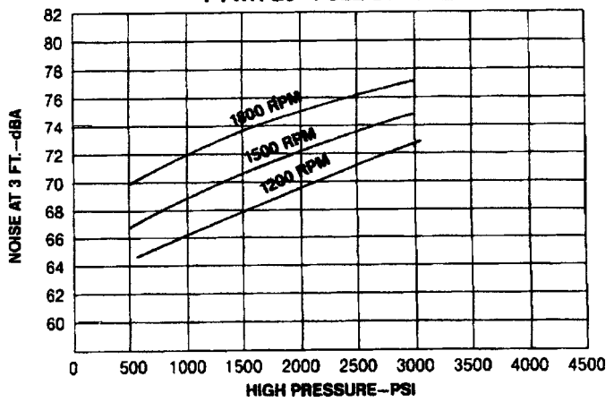
PVWH-20—FULL STROKE
