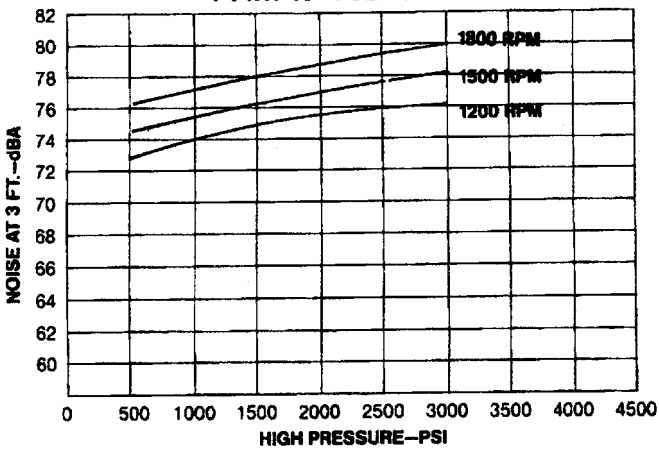
PVWH-45—FULL STROKE
