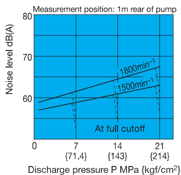
Noise Characteristics
