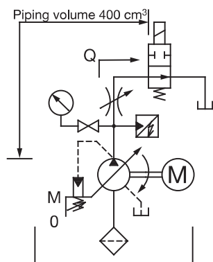
Test Circuit
