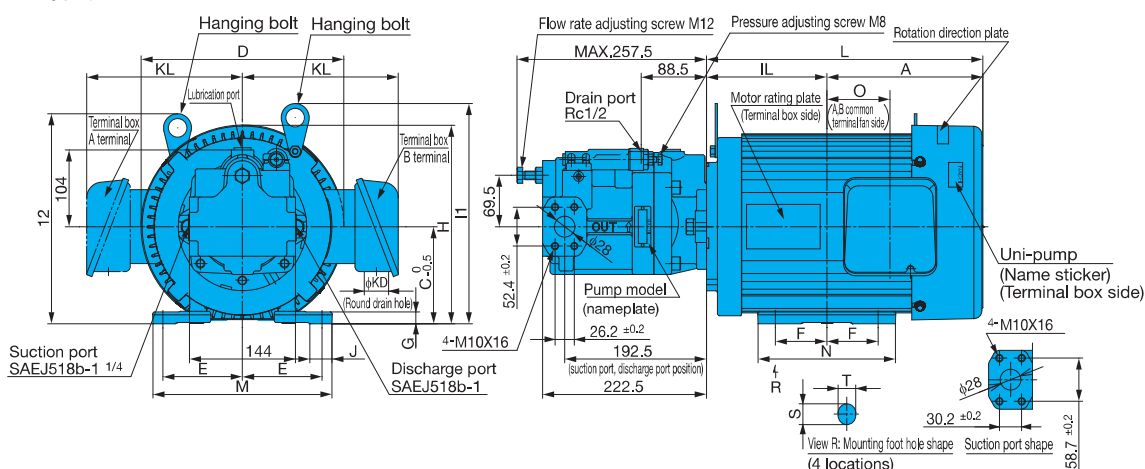
UPV-2A-35 35 45 -**-**-4-30 (side port type)
