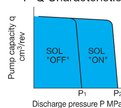
P-Q Characteristics
