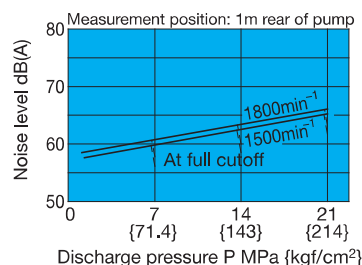
Noise Characteristics
