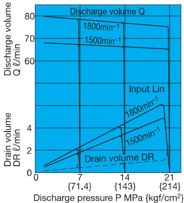
Pressure - Discharge Volume Characteristics
