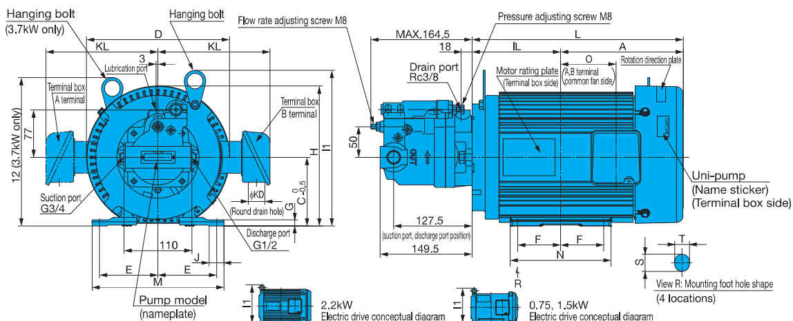
UPV-1A-16 16 22 -**-**-4-30 (side port type)
