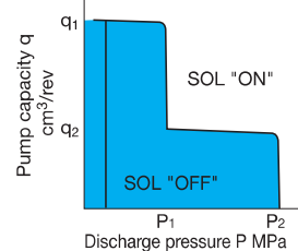
P-Q Characteristics
