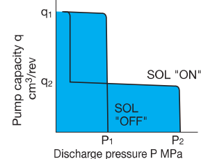
P-Q Characteristics
