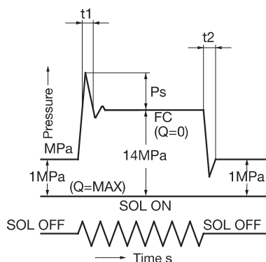
Graph Legend
