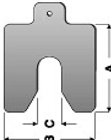
Shim Size
