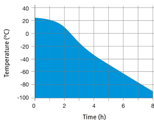
Pull-down time
