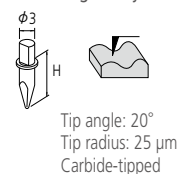
Intersecting cut stylus
