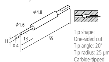
Small hole stylus SPH-42
