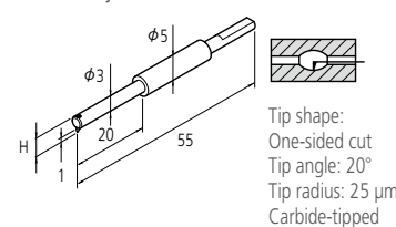
Small hole stylus SPH-43
