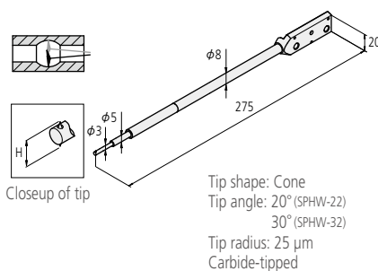
| Double-sided Small Hole Arm Stylus SPHW-22/32
