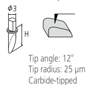
One-sided cut stylus
