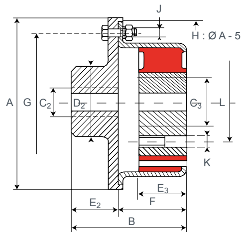
Solid hub coupling
