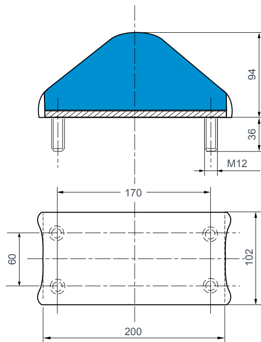
reference 519186 defection : 35 mm maximal charge : 3 000 daN
