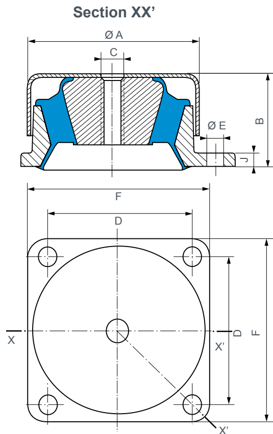
STABIFLEX - square base
