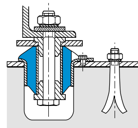
Shape 3 - Fixing between the equipment and concrete (using locating rings).
