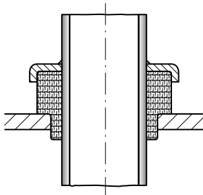
Pipe isolation
