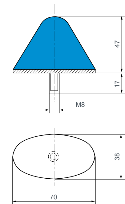
reference 512389 defection : 14 mm maximal charge : 150 daN
