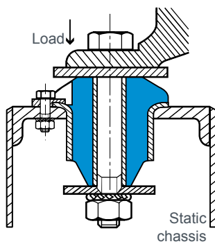
Shape 1 - Fixing between the equipment and a metallic chassis (failsafe in mobile applications).
