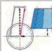
Taper cutting
