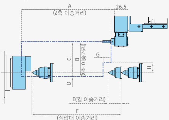
Angular Milling Holder
